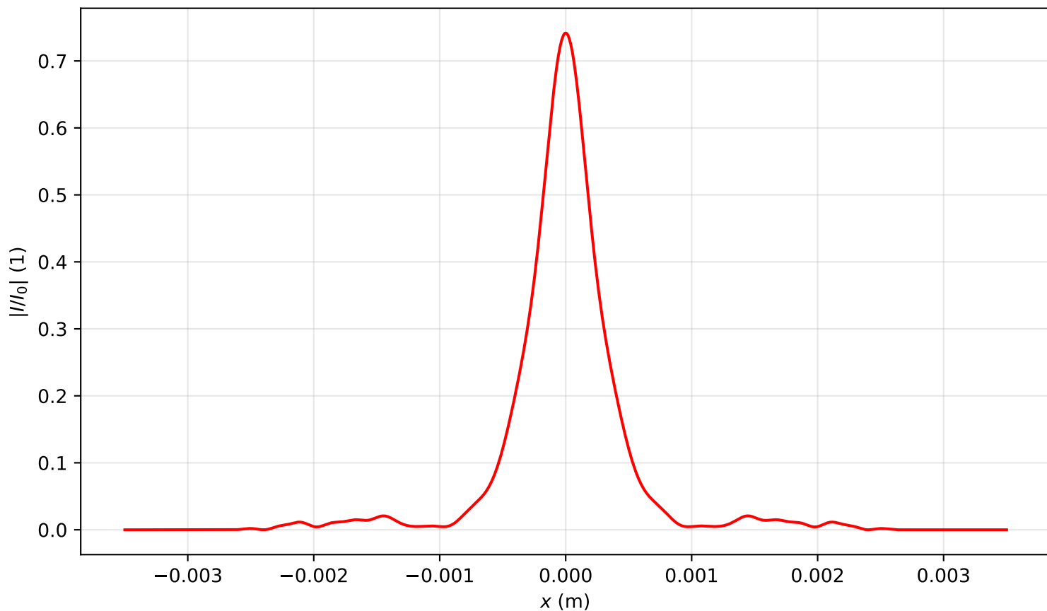
Intensity profile I(x, y = 0, z = 3.821)/I_0 , P_{in}=3.0P_{cr} , artificial time
